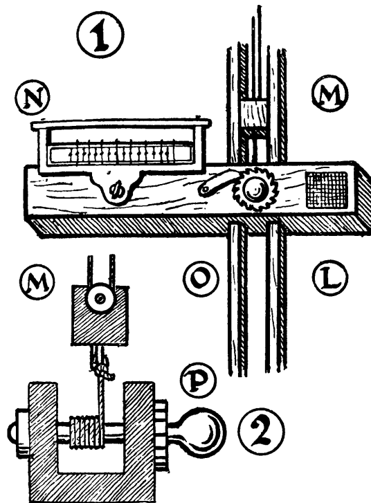
FIG. 23.—The Heck-block.
