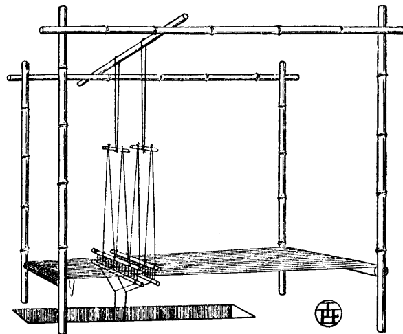
FIG. 41.—Indian Loom.
