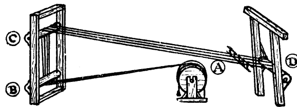
FIG. 38.—Beaming in a Smaller Space.
