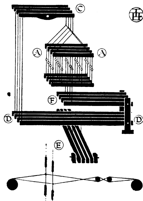
FIG. 85A.—Shedding Motion.
