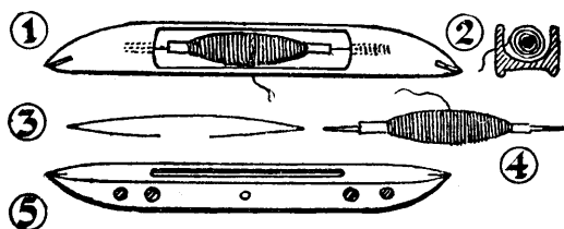
FIG. 51.—Hand-shuttle.
