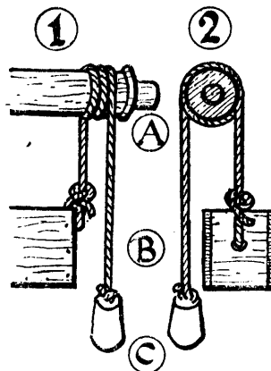
FIG. 43.—Cane Roller and Weighting.
