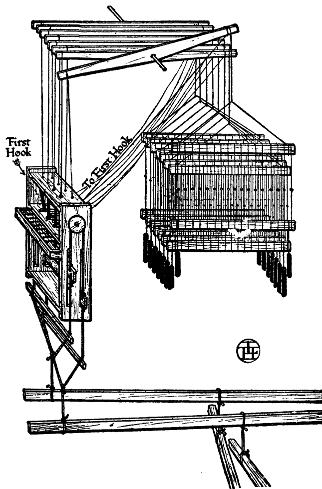
FIG. 97.—The Jack-in-the-box.
