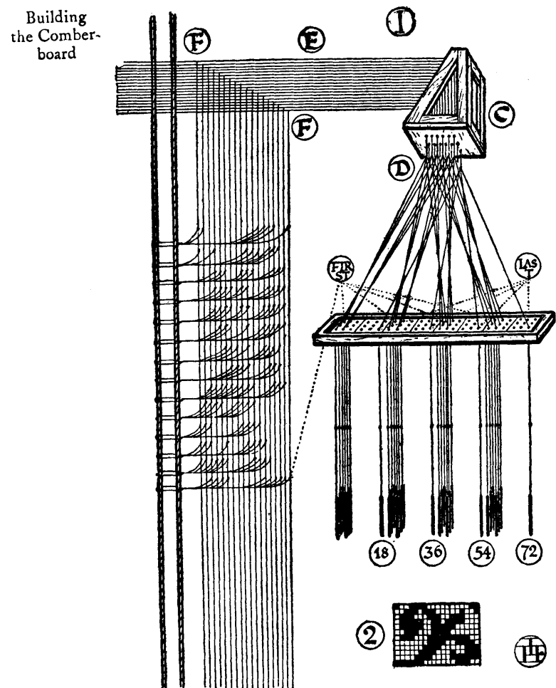
FIG. 105 —Mechanism of the Draw-loom.
