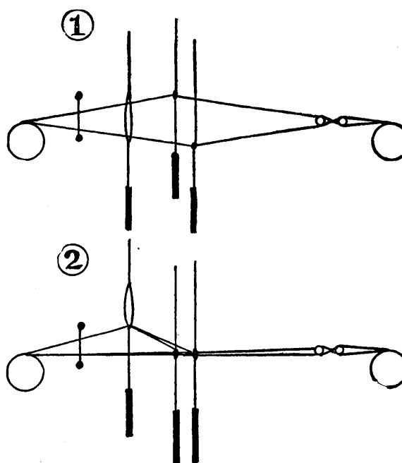
FIG. 66.—Section of Two Sorts of Leashes.
