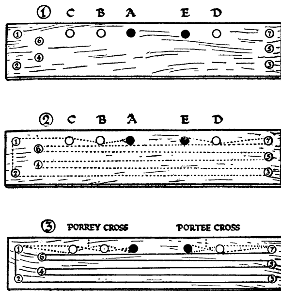
FIG. 14.—Warping Board.
