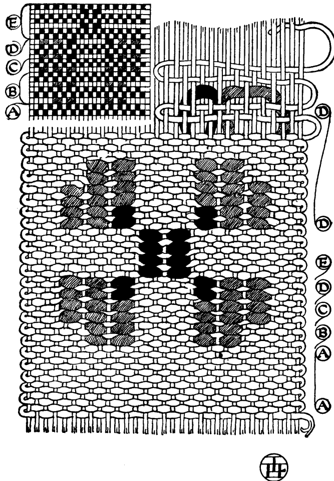
FIG. 64.—Brocading on Board.
