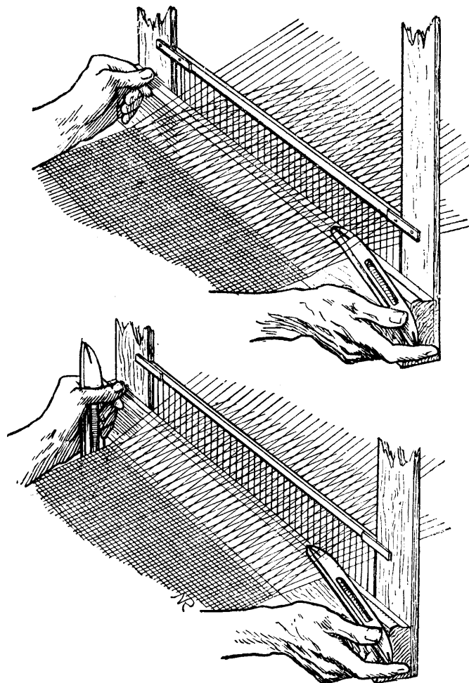
FIG. 52.—Method of handling One, or Two, Shuttles. If more than two shuttles are used they are laid in order on the web.
