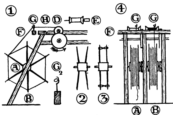
FIG. 14. WINDING MACHINE
