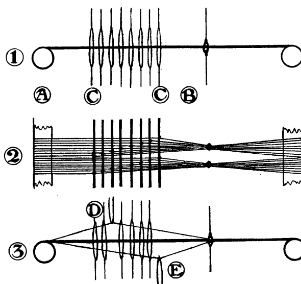
FIG. 36. DIAGRAM OF DOUBLE HARNESS
