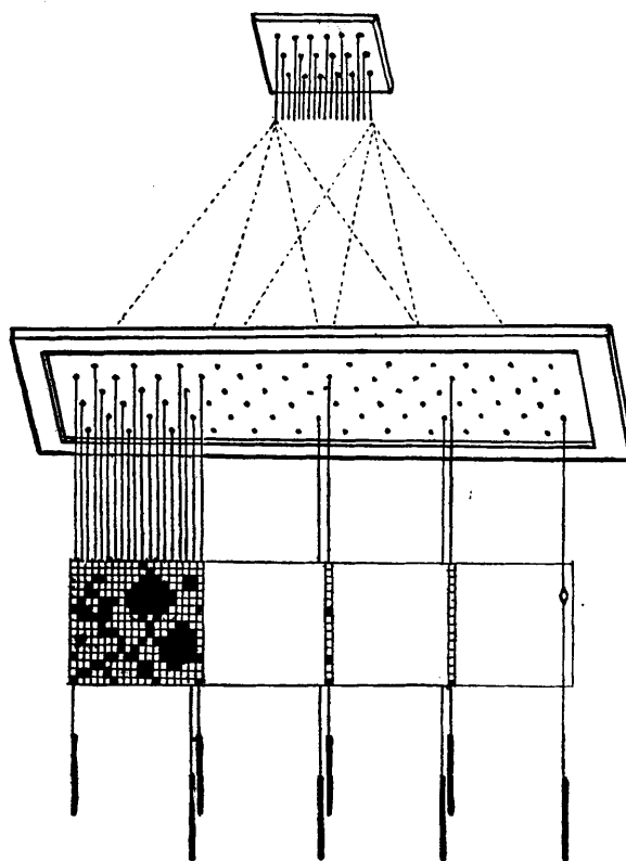
FIG. 32. DRAW-LOOM MONTURE
