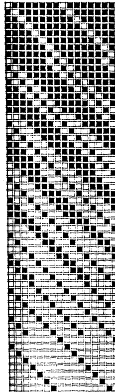
FIG. 103. 8-HARNES TWILL.
