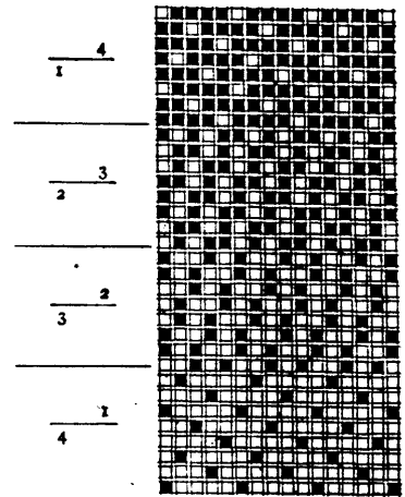
FIG. 100.—5-LEAF SATIN.
