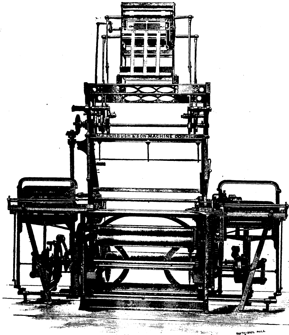
MURKLAND HIGH SPEED INGRAIN CARPET LOOM. M. A. FURBUSH & SON MACHINE CO., PHILADELPHIA.
